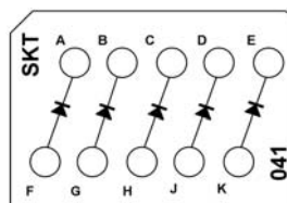
CTJ420E041 Five JANTX 1N5550 Diodes
