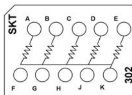
CTJ420E302 Four 2.7 k Resistors, 1/4 W One 3.9 k Resistor, 1/4 W
