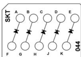
CTJ420E044 Five JANTX 1N5552 Diodes
