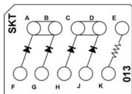
CTJ420E013 Four JANTX 1N5618 Diodes One 200 Resistor, 1/8 W
