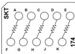
CTJ420E174 Five 100 k Ohm Resistors, 1/10 W
