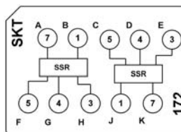
CTJ420E172 Two TELEDYNE M93F-1 ISO Cubes
