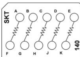
CTJ420E140 Five 5.1 k Resistors, 1/10 W
