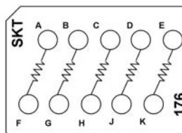
CTJ420E176 Five 470 Ohm Resistors, 1/2 W
