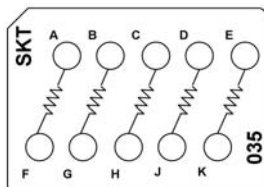
CTJ420E035 Five 10.2 k Resistors, 1/10 W
