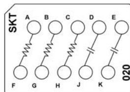
CTJ420E020 Two 3.6 k Resistors, 1/10 W One 100 k Resistor, 1/10 W Two 1 µF Capacitors, 50 WVDC
