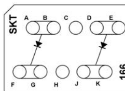
CTJ420E166 Two ON Semiconductor MR756 Diodes
