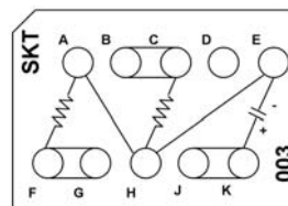
CTJ420E003 Two 150 Resistors, 1/4 W One 10 \mu F Capacitor, 35 WVDC
