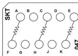
CTJ420E047 Three 60.4 Resistors, 2 W
