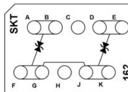
CTJ420E162 Two JANTX 1N6067A Zener Diodes
