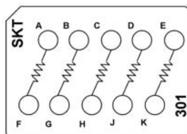
CTJ420E301 Four 2.7 k Resistors, 1/4 W One 56 Resistor, 1/2 W
