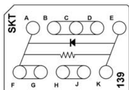
CTJ420E139 One 1 k Resistor, 1 W One JANTXV 1N5550 Diode
