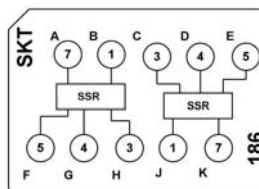
CTJ420E186 Two TELEDYNE M92F-3 ISO Cubes
