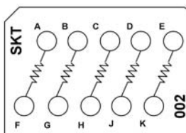
CTJ420E002 Five 150 Resistors, 1/4 W
