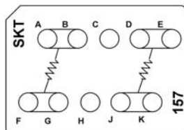
CTJ420E157 Two 120 Ohm Resistors, 1/4 W
