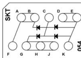
CTJ420E054 Four JANTXV 1N5416 Diodes
