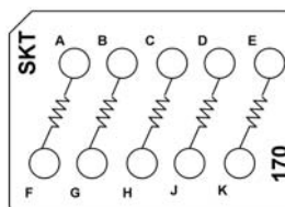
CTJ420E170 Five 249 Ohm Resistors, 1/4 W
