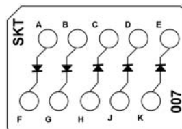
CTJ420E007 Three JAN 1N3613 Diodes Two JAN 1N645 Diodes
