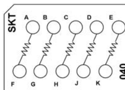
CTJ420E040 Five 49.9 k Resistors, 1/20 W
