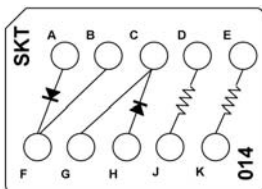
CTJ420E014 Two JANTX 1N5618 Diodes Two 10 k Resistors, 1/10 W
