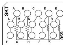
CTJ420E059 Four 150 Resistors, 1/4 W
