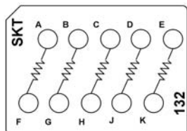
CTJ420E132 Five 150 Ohm Resistors, 1/2 W
