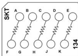
CTJ420E134 Three 150 Ohm Resistors, 1/2 W One 51 Ohm Resistor, 1/2 W One 820 Ohm Resistor, 2 W
