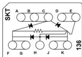
CTJ420E136 Four JANTX 1N5619 Diodes One 200 k Resistor, 1/2 W
