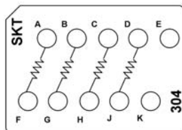
CTJ420E304 Two 120 Resistors, 1/2 W Two 2.7 k Resistors, 1/4 W
