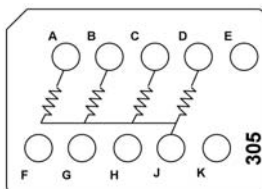
CTJ420E305 Two 2.7 k Resistors, 1/4 W Two 3.9 k Resistors, 1/4 W
