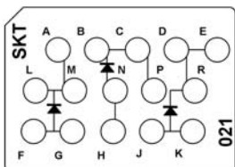
CTJ420E021 Three JANTX 1N5550 Diodes
