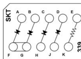
CTJ420E339 One 100 Resistor, 1/2 W Four JANTX 1N3613 Diodes
