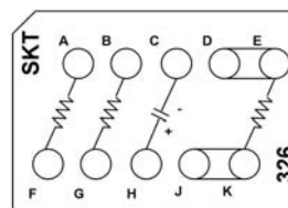
CTJ420E326 One 100 Resistor, 1/4 W One 300 Resistor, 1/4 W One 573 Resistor, 1/4 W One 10 μF Capacitor, 35 WVDC
