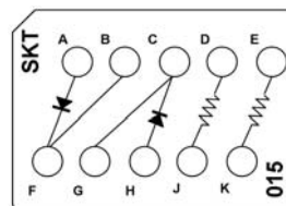
CTJ420E015 Two JANTX 1N5618 Diodes One 10 k Resistor, 1/10 W One 110 Resistor, 1/10 W
