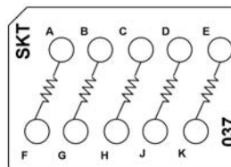
CTJ420E037 Five 23.2 k Resistors, 1/20 W
