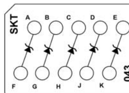
CTJ420E043 Five JANTX 1N827 Zener Diodes
