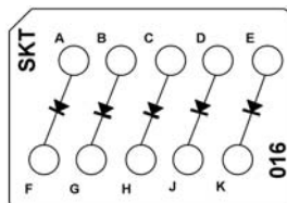
CTJ420E016 Five JANTX 1N5618 Diodes
