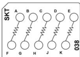
CTJ420E038 Five 24.9 k Resistors, 1/20 W
