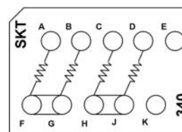
CTJ420E340 Two 2.2 k Resistors, 1/2 W Two 240 k Resistors, 1/2 W
