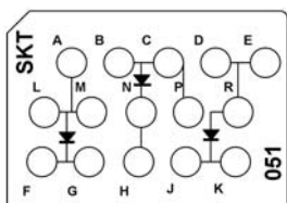
CTJ420E051 Three JANTX 1N5618 Diodes
