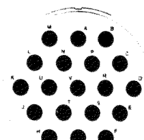
25-19 19 SIZE 12 CONTACTS
