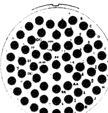
25-61 61 SIZE 20 CONTACTS
