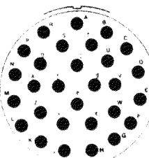
25-29 29 SIZE 16 CONTACTS
