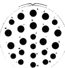
25-24 12 SIZE 12 CONTACTS 12 SIZE 16 CONTACTS
