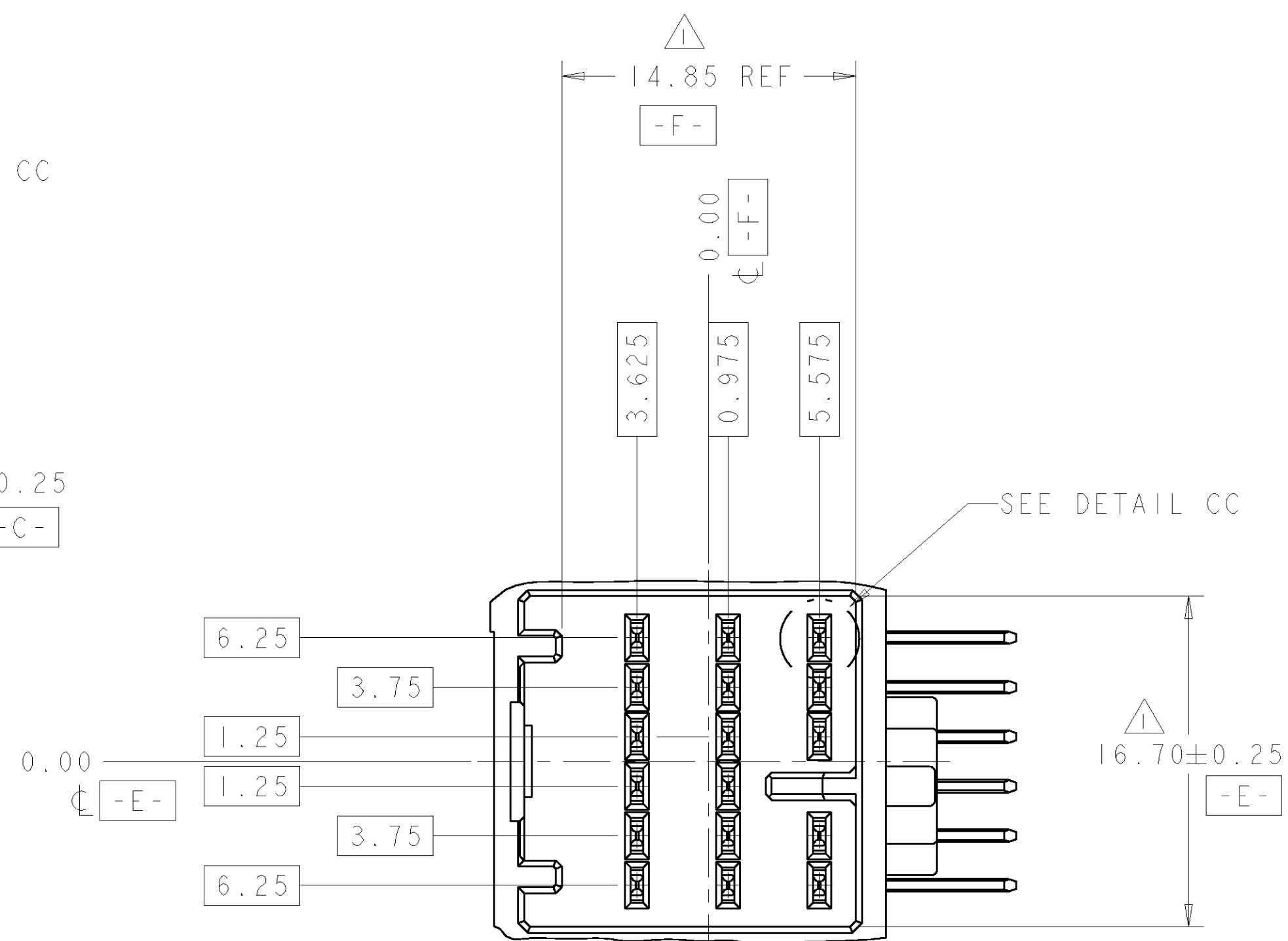
DETAIL WW SCALE 4:1
