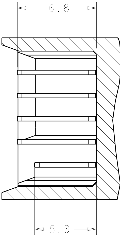
SECTION KB-KB △5 (LEVEL 12222: LEVEL 1 ROW "A" ONLY LEVEL 2 ROWS "B" THRU "E")
