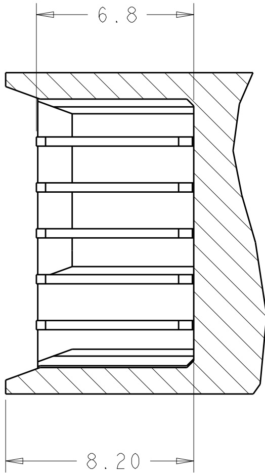
SECTION LL-LL △5 (LEVEL 2: ALL LONGEST CONTACT)
