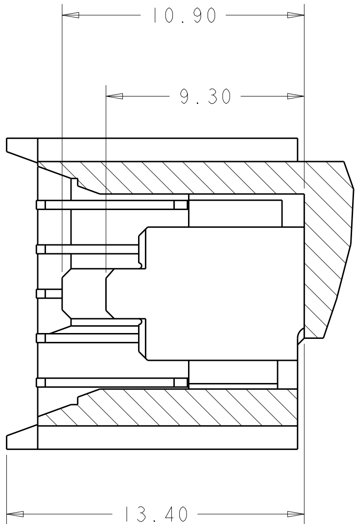
SECTION R-R △5 (LEVEL 2, SHORTEST, & LEVEL 3 LONGEST, MATING CONTACTS)
