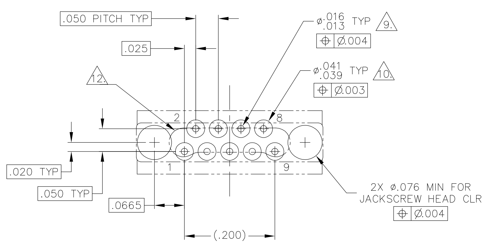
TYPICAL PCB LAYOUT SIZE 09 SHOWN FOR REFERENCE
