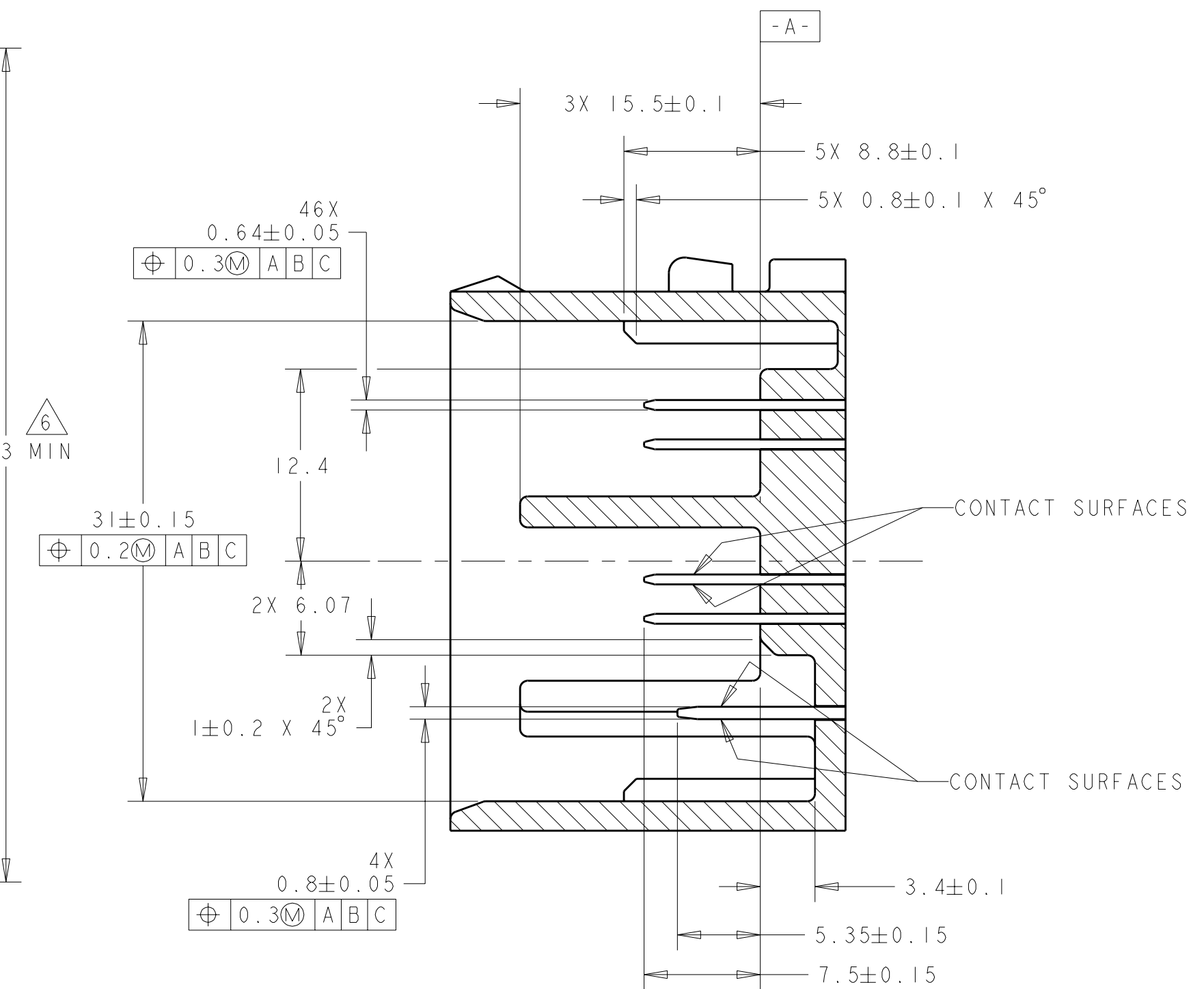
SECTION B-B
