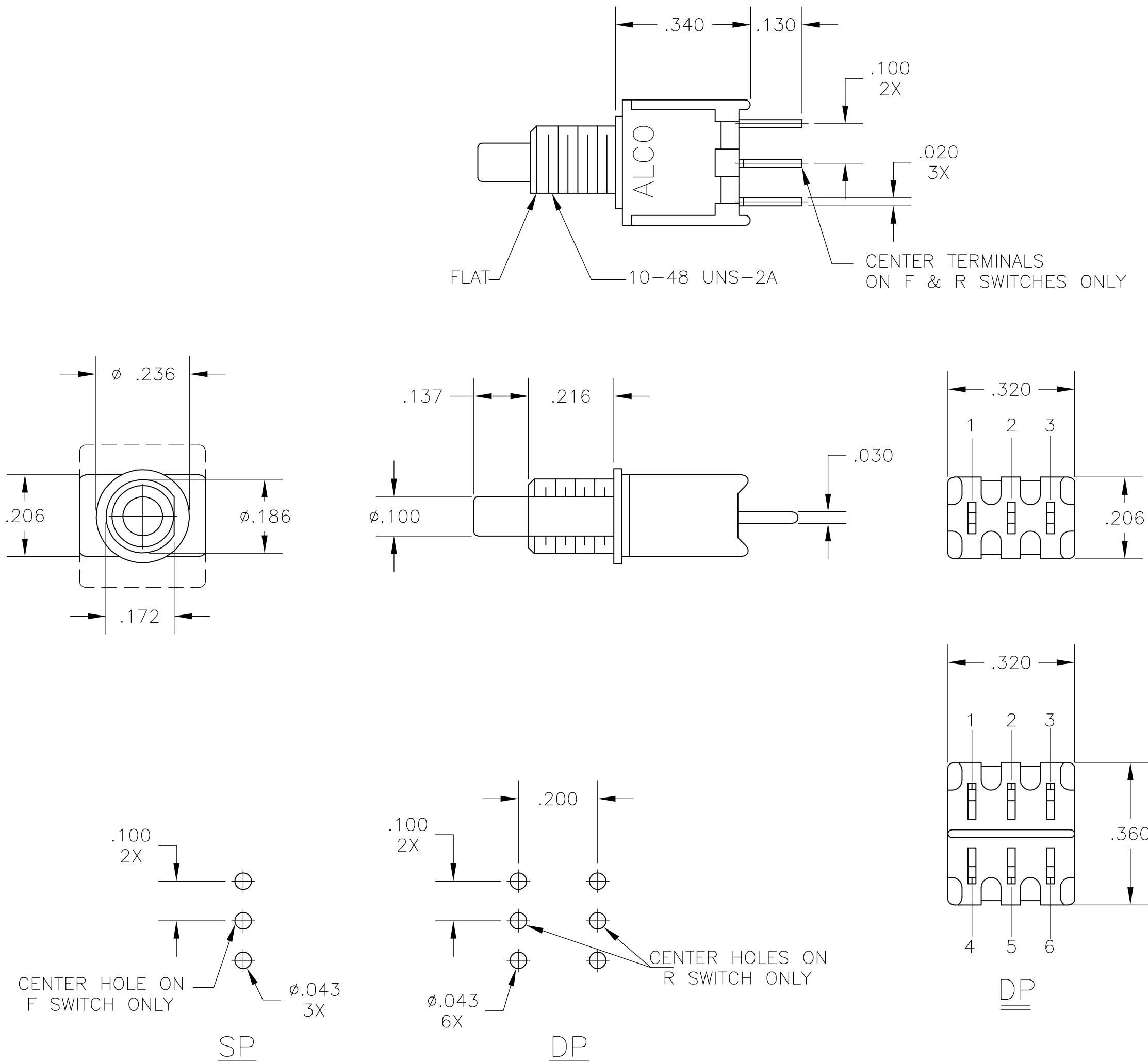
RECOMMENDED HOLE LAYOUT TOLERANCE ±.002 UNLESS OTHERWISE NOTED
