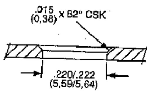
Figure A Recommended Chassis Cutout for all 8060 Series panel mount applicaions
