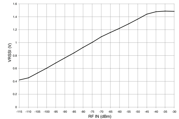
Figure 7: RSSI Curve
