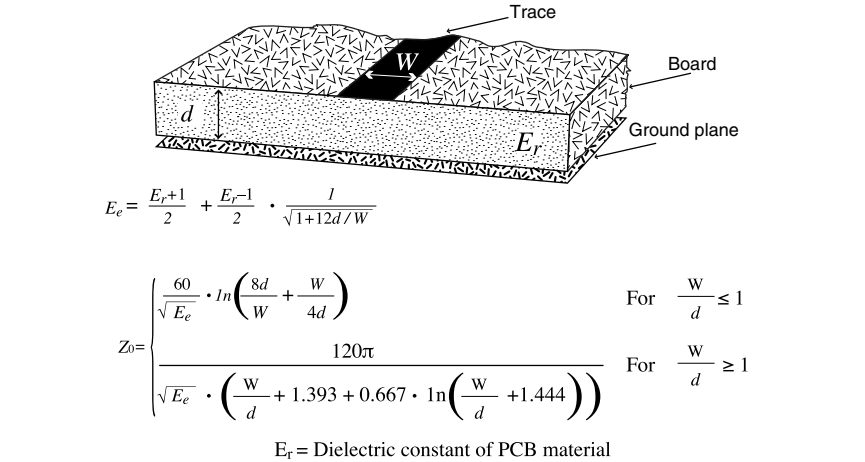
Figure 20: Microstrip Formulas
