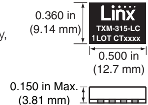
Figure 1: Package Dimensions
