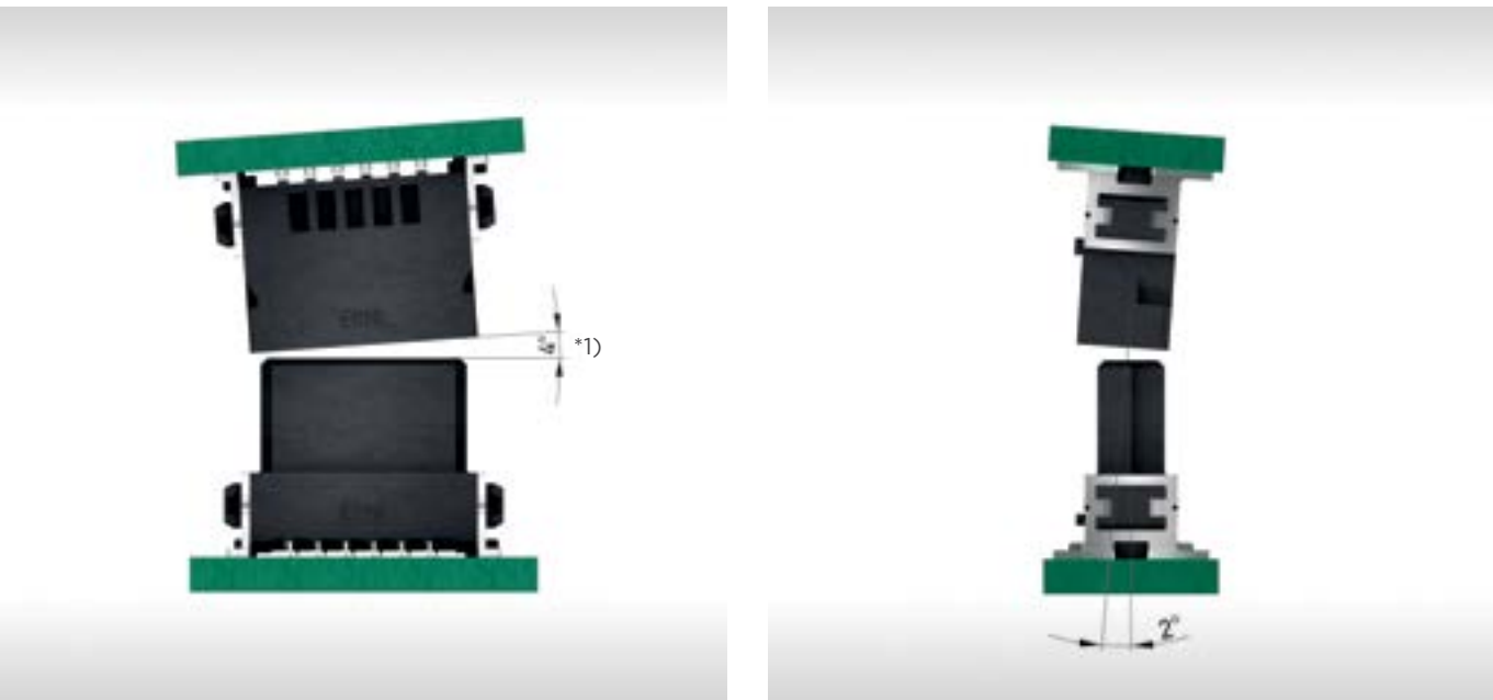
Allowed Inclination for a more Secure Self-Centering
