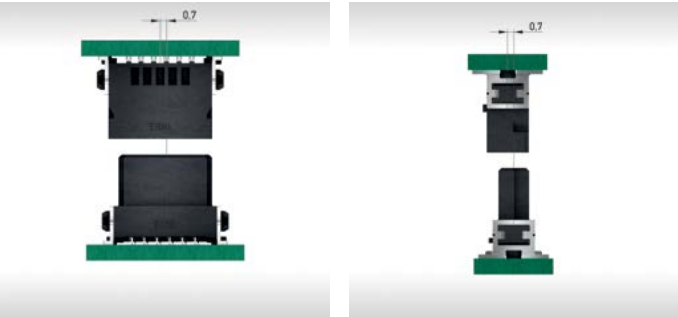
Allowed Misalignment Tolerances for a more Secure Self-Centering
