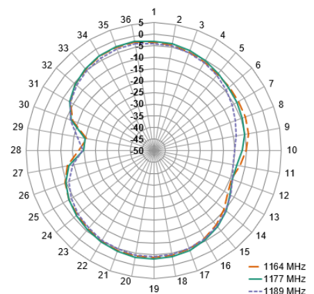
XY-Plane Gain
