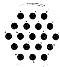
25-19 19 SIZE 12 CONTACTS
