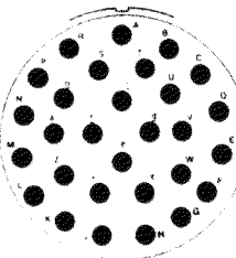
25-29 29 SIZE 16 CONTACTS
