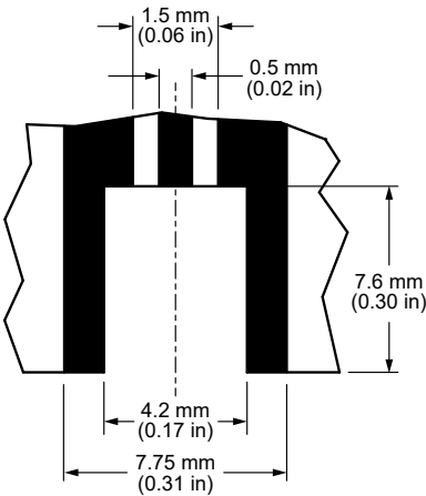
Figure 2. Recommended PCB Dimensions for the CONSMP024-G
