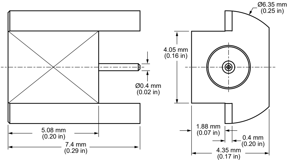
Figure 1. Product Dimensions for the CONSMP024-G Connector Table
