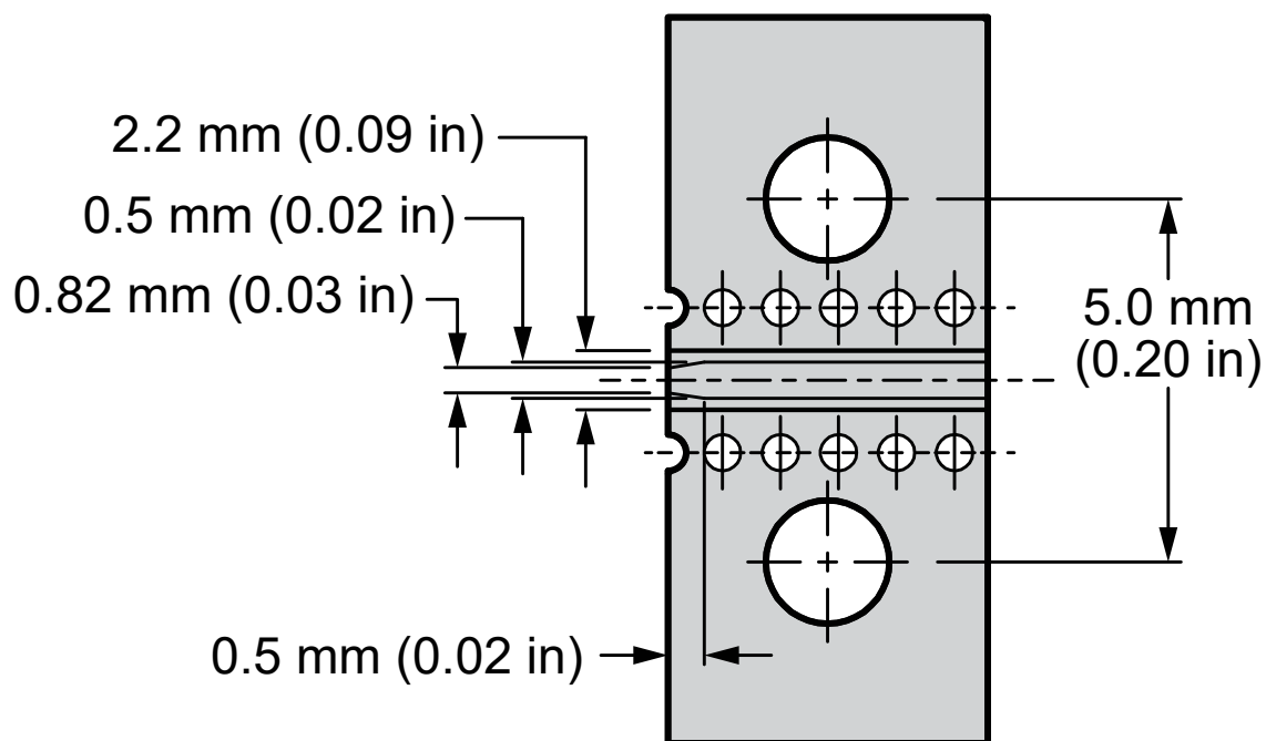
Figure 2: Recommended PCB Dimensions for the CON292003
