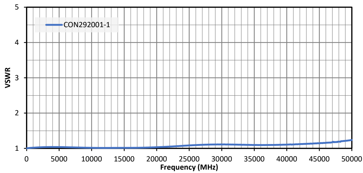
Figure 4: VSWR for the CON292001-1 Connector
