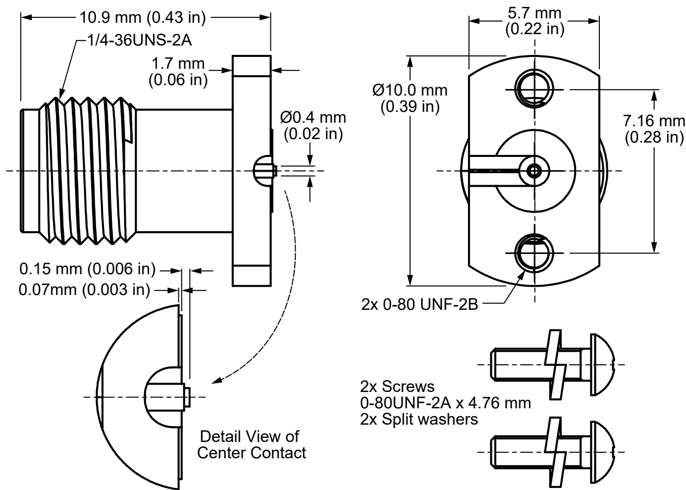
Figure 1: Product Dimensions for the CON292001-1 Connector
