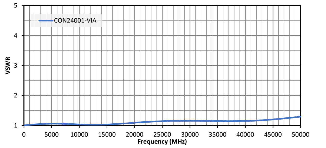
Figure 4: VSWR for the CON24001-VIA Connector
