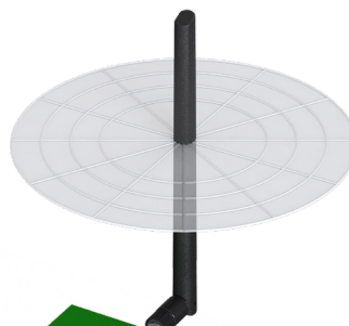
XY-Plane Gain
