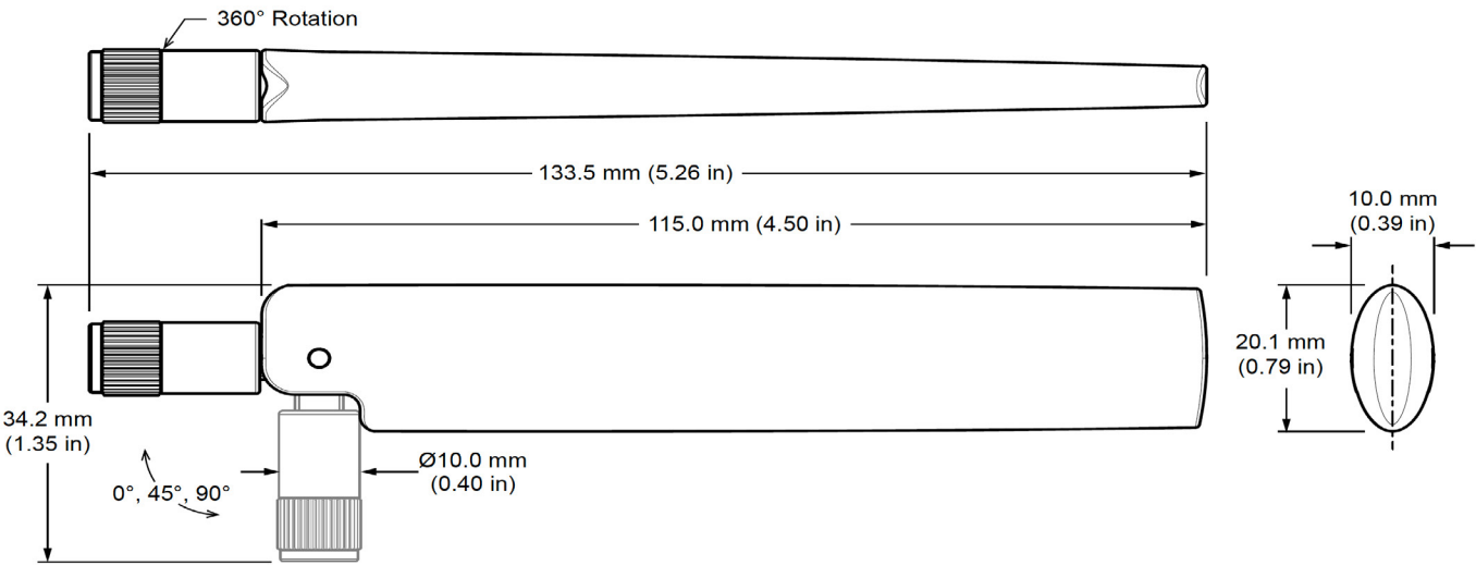
Figure 1. ANT-W63WS2-ccc Antenna Dimensions
