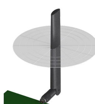
XY-Plane Gain
