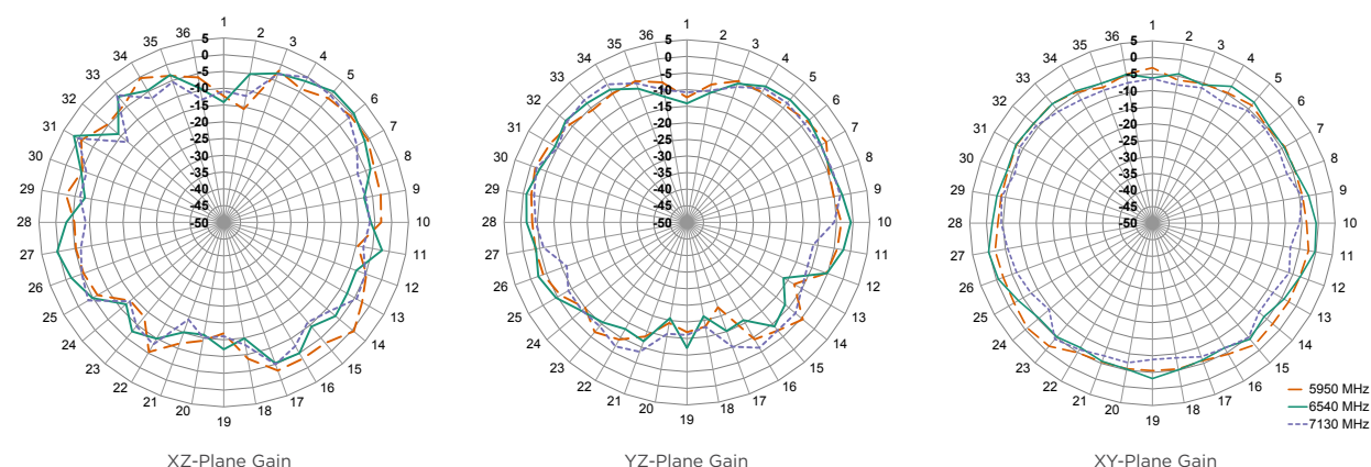
Figure 9. Radiation Patterns for ANT-W63WS2-ccc, Edge-Bent
