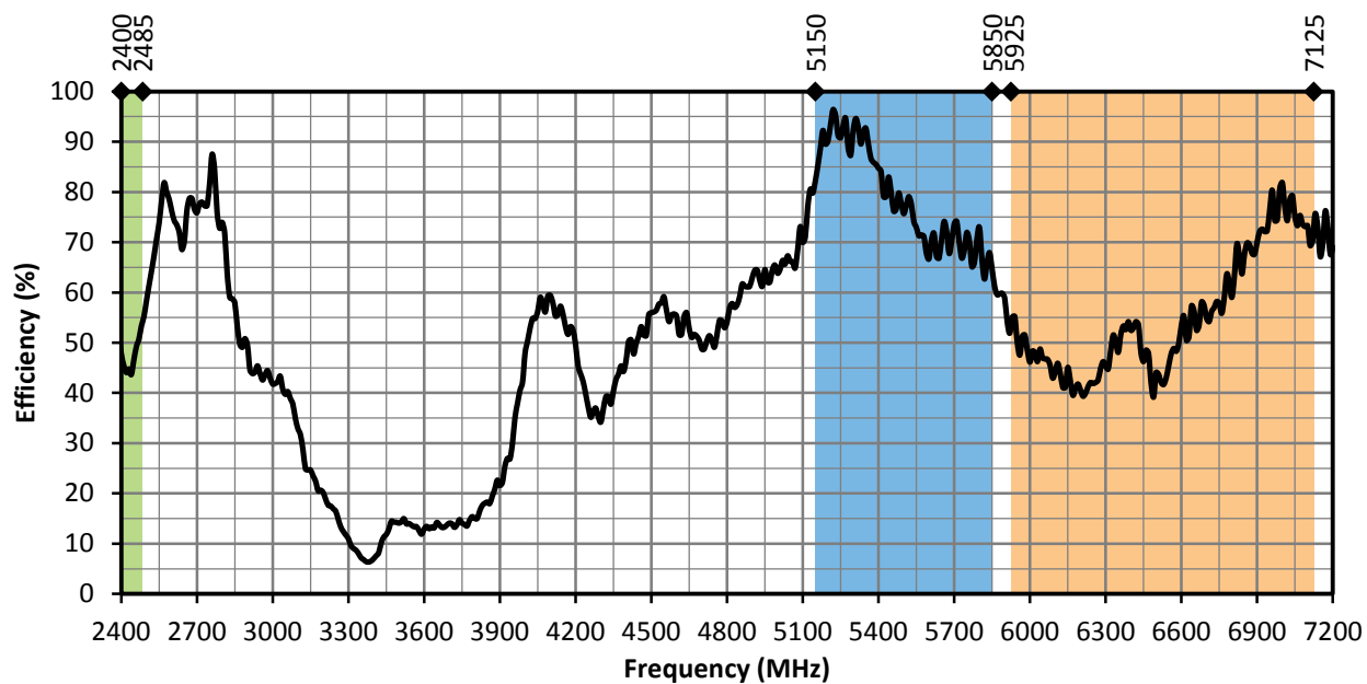
Figure 9. ANT-W63-WRT Series Antenna Radiation Efficiency, Free Space
