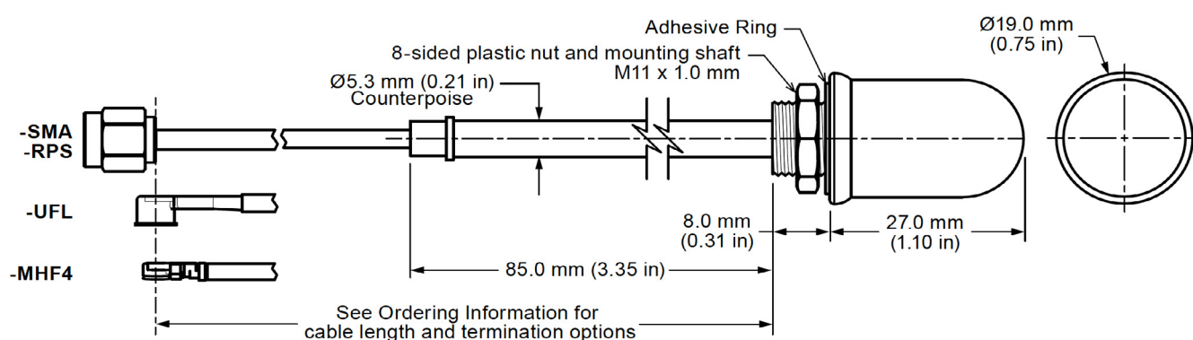
Figure 1. ANT-W63-WRT-ccc Antenna Dimensions
