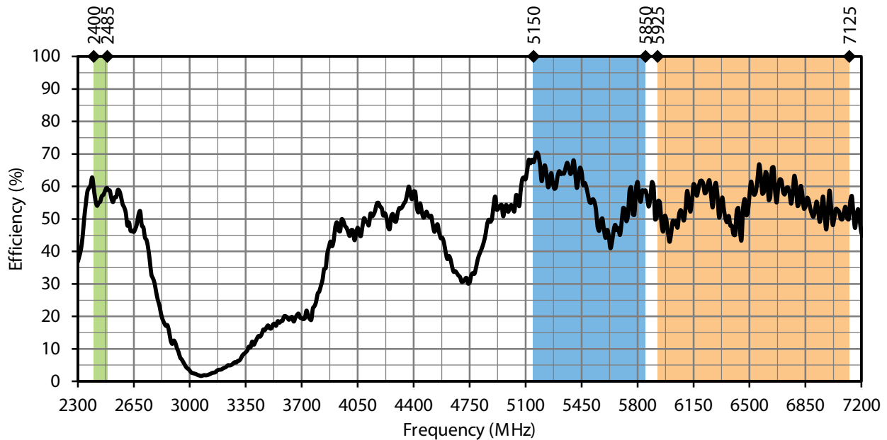
Figure 8. W63WS1 Series Antenna Radiation Efficiency, Straight
