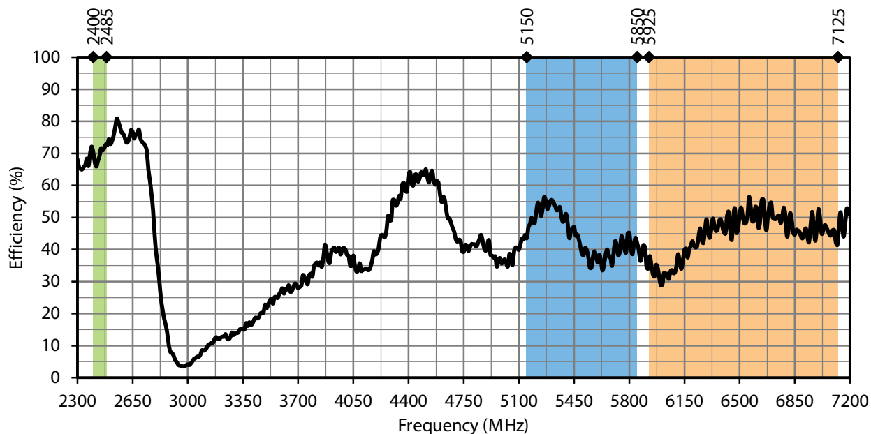
Figure 15. W63WS1 Antenna Radiation Efficiency, Edge-Bent
