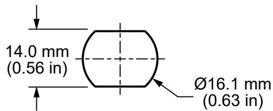
Figure 2: ANT-W63-SPNF1 Mounting Hole Dimensions
