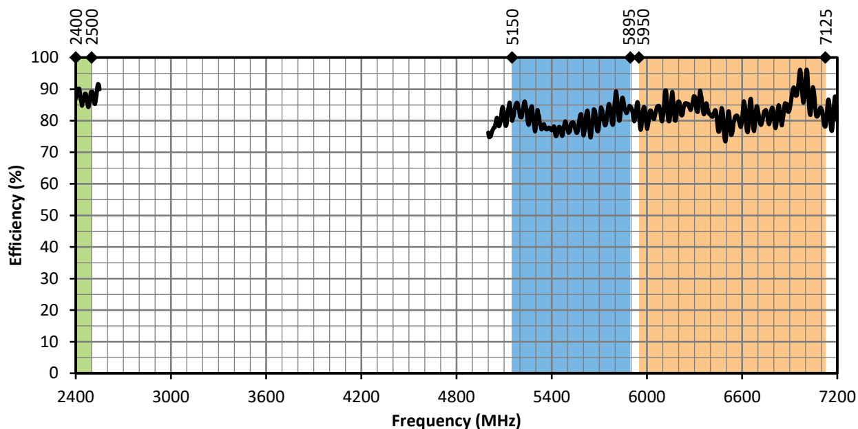
Figure 7: ANT-W63-SPNF1 Antenna Efficiency with Frequency Band Highlights
