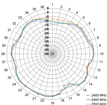
XY-Plane Gain
