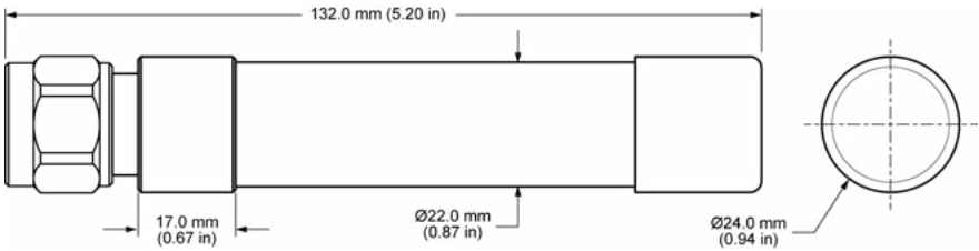
Figure 1. ANT-W63-IPW2-NP Antenna Dimensions
