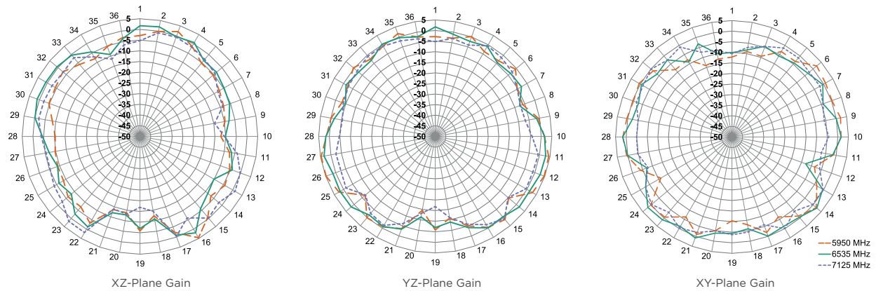
Figure 9. ANT-W63-CW-RCS-ccc Radiation Patterns, Free Space
