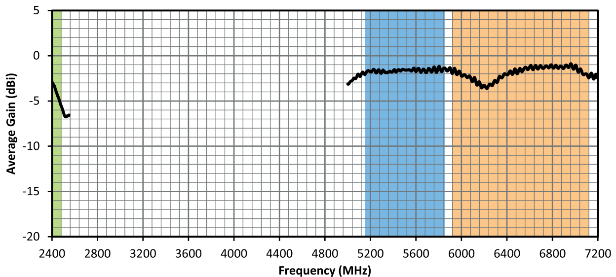
Figure 7. ANT-W63-CW-RCS-ccc Antenna Average Gain, Free Space
