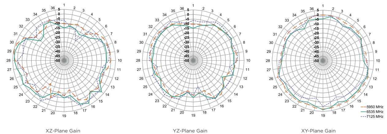
Figure 16. Radiation Patterns for ANT-W63-CW-RCS-ccc, on Edge of Ground Plane
