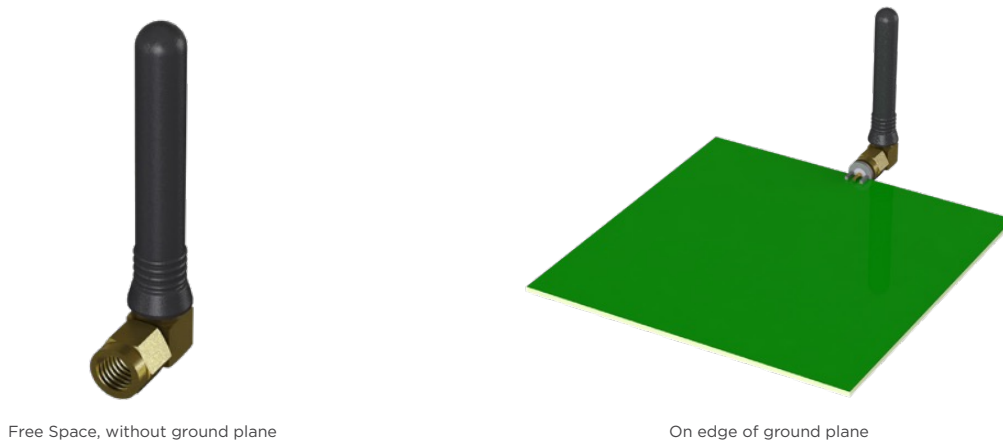
Figure 2. ANT-W63-CW-RCS-ccc Test Orientation
