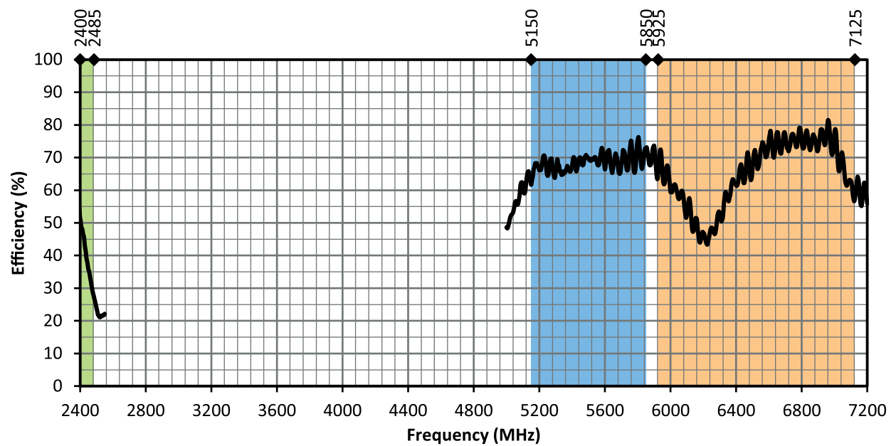
Figure 8. ANT-W63-CW-RCS-ccc Antenna Radiation Efficiency, Free Space
