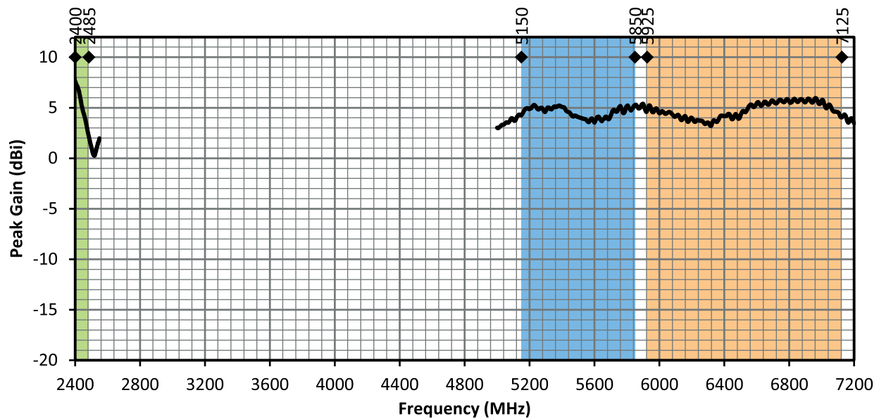
Figure 6. ANT-W63-CW-RCS-ccc Peak Gain, Free Space
