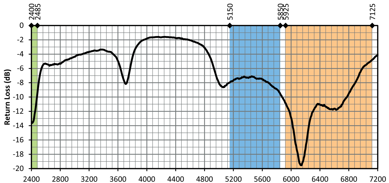
Figure 12. ANT-W63-CW-RCS-ccc Return Loss, on Edge of Ground Plane
