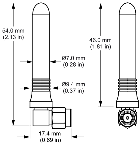
Figure 1. ANT-W63-CW-RCS-ccc Antenna Dimensions
