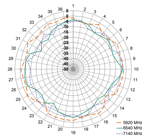
XY-Plane Gain
