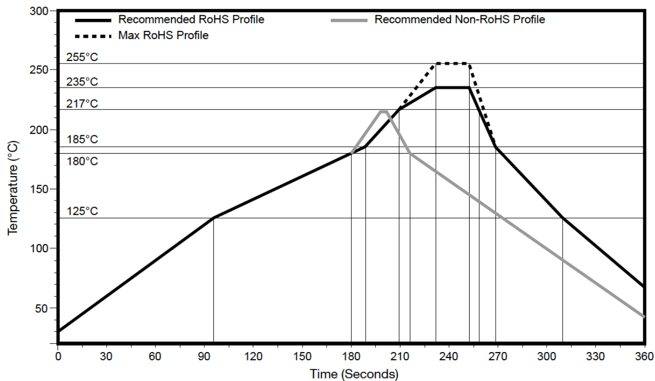
Figure 11. Solder Profile for the ANT-915-VHETH Antenna
