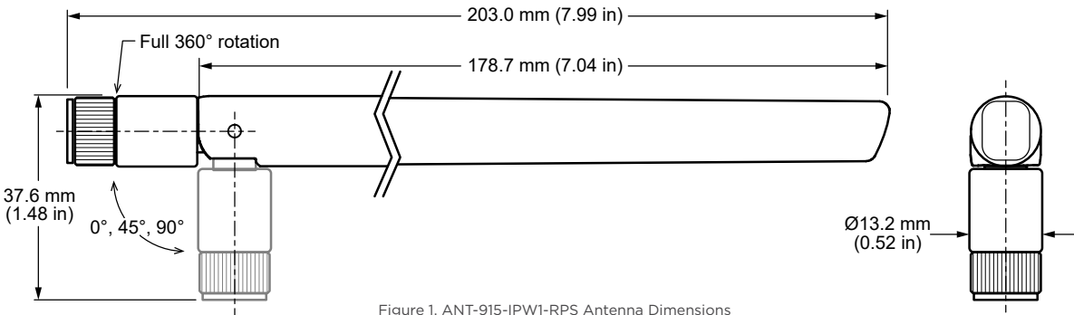
Figure 1. ANT-915-IPW1-RPS Antenna Dimensions
