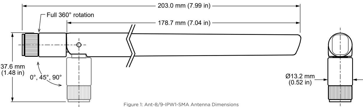
Figure 1: Ant-8/9-IPW1-SMA Antenna Dimensions
