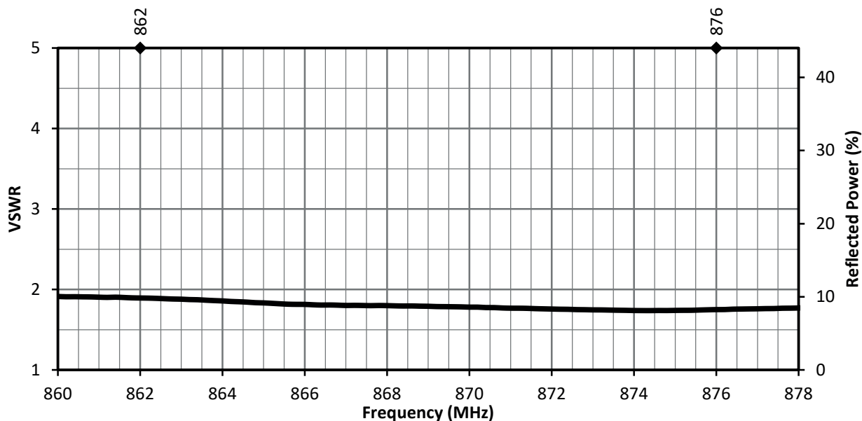
Figure 3. ANT-868-CW-RCL VSWR
