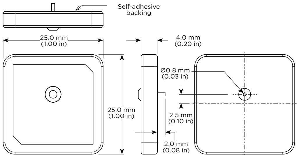
Figure 1. 868-CPA Antenna Dimensions
