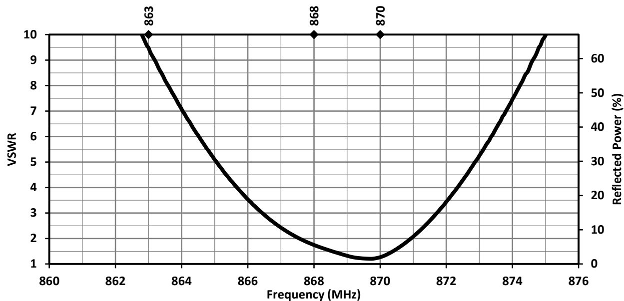
Figure 2. 868-CPA VSWR
