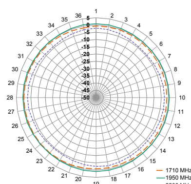
XY-Plane Gain
