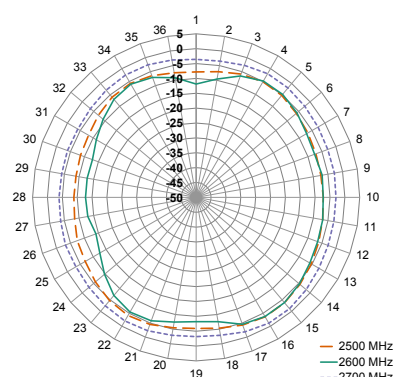
XY-Plane Gain
