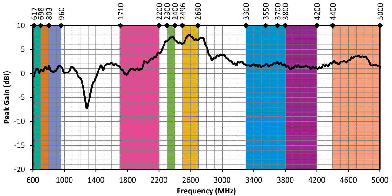
Figure 6. ANT-5GW-IPW2-NP Peak Gain, Free Space
