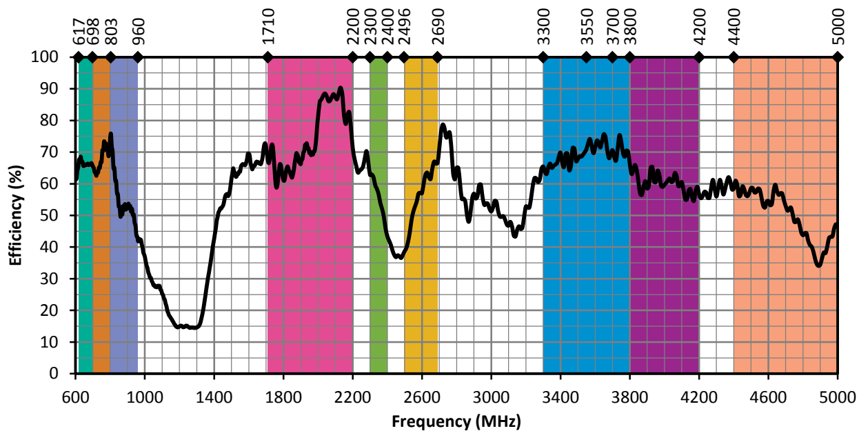
Figure 15. ANT-5GW-IPW2-NP Antenna Efficiency, Center of Ground Plane
