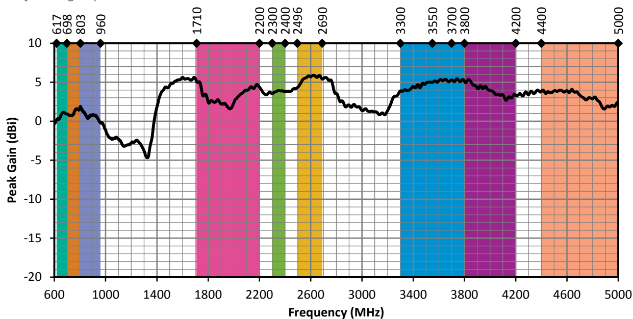
Figure 13. ANT-5GW-IPW2-NP Peak Gain, Center of Ground Plane
