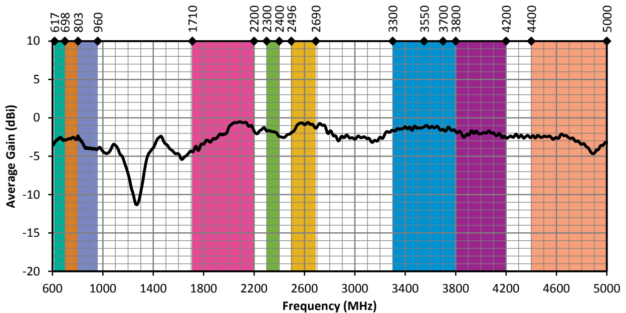
Figure 7. ANT-5GW-IPW2-NP Antenna Average Gain, Free Space
