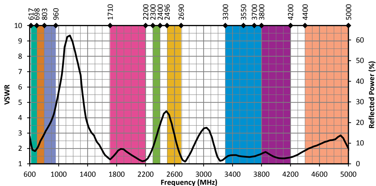
Figure 11. ANT-5GW-IPW2-NP VSWR, Center of Ground Plane
