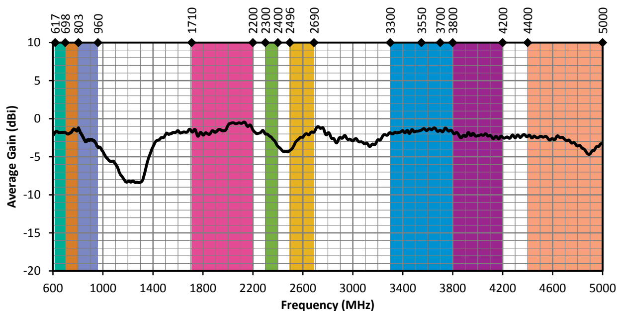
Figure 14. ANT-5GW-IPW2-NP Antenna Average Gain, Center of Ground Plane
