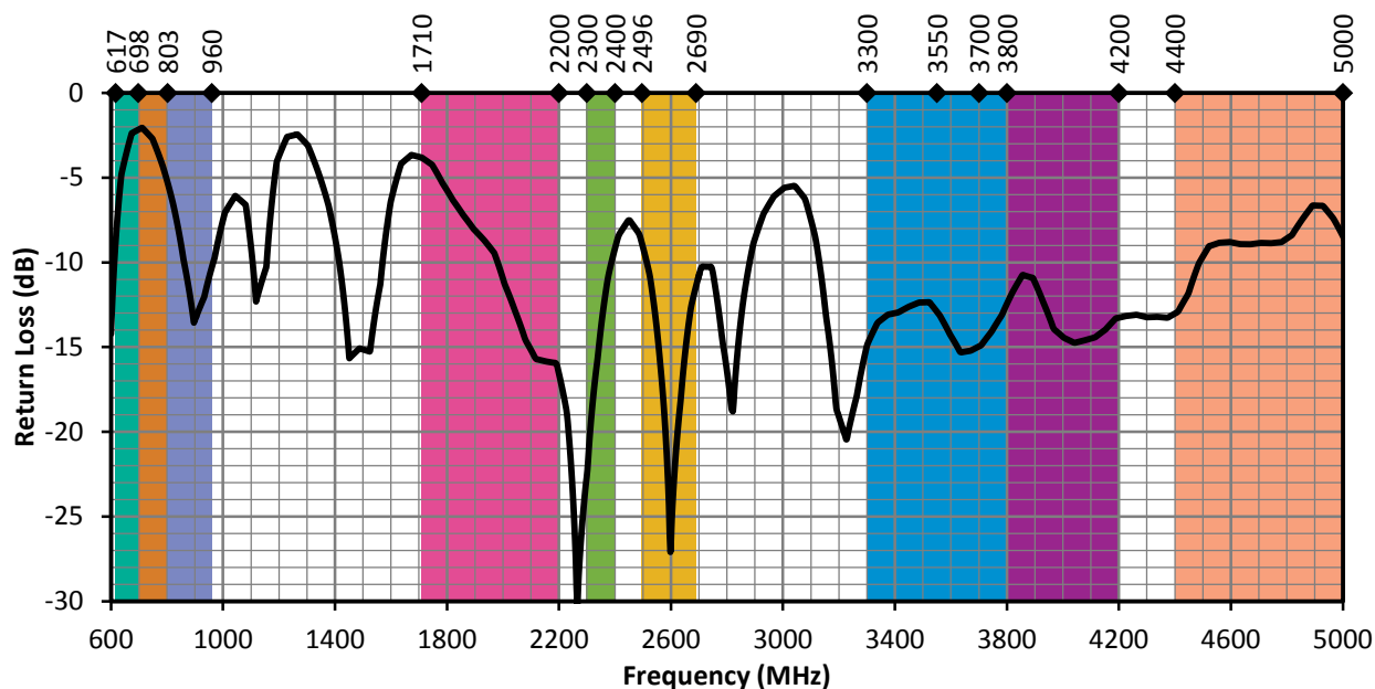
Figure 5. ANT-5GW-IPW2-NP Return Loss, Free Space
