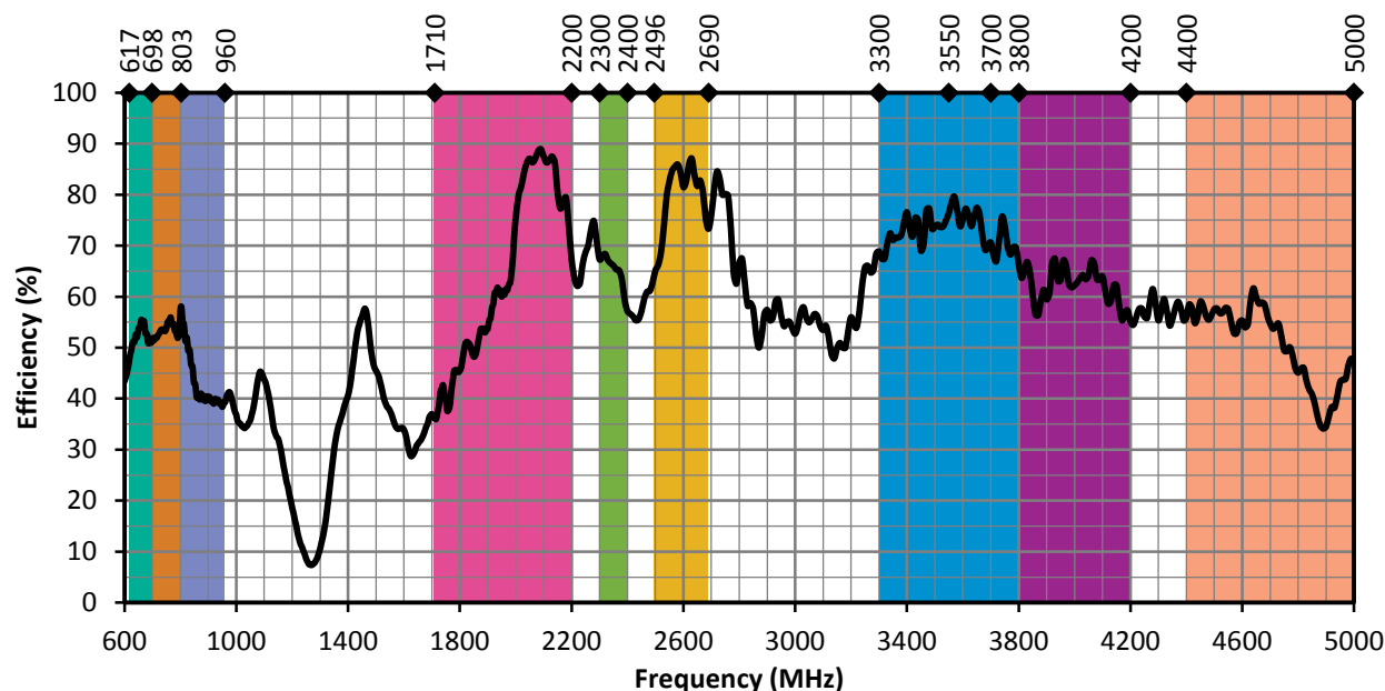
Figure 8. ANT-5GW-IPW2-NP Antenna Efficiency, Free Space
