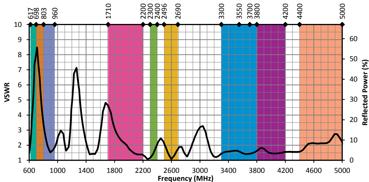
Figure 4. ANT-5GW-IPW2-NP VSWR, Free Space
