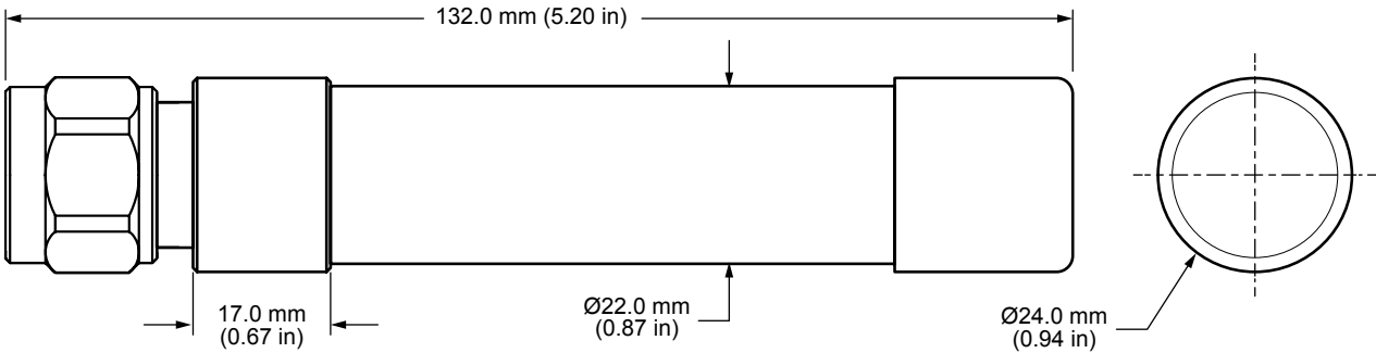
Figure 1. ANT-5GW-IPW2-NP Antenna Dimensions
