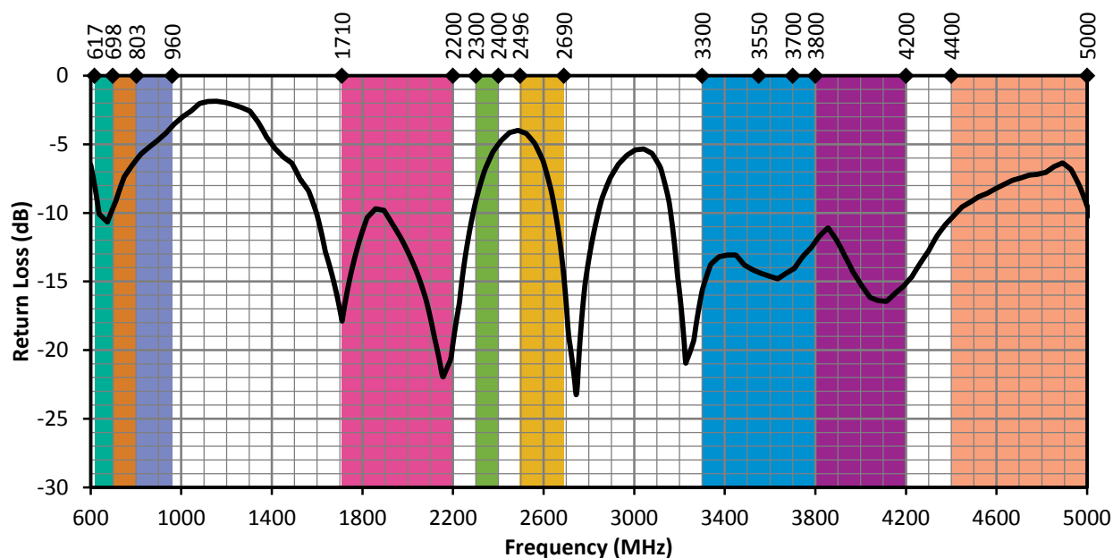
Figure 12. ANT-5GW-IPW2-NP Return Loss, Center of Ground Plane
