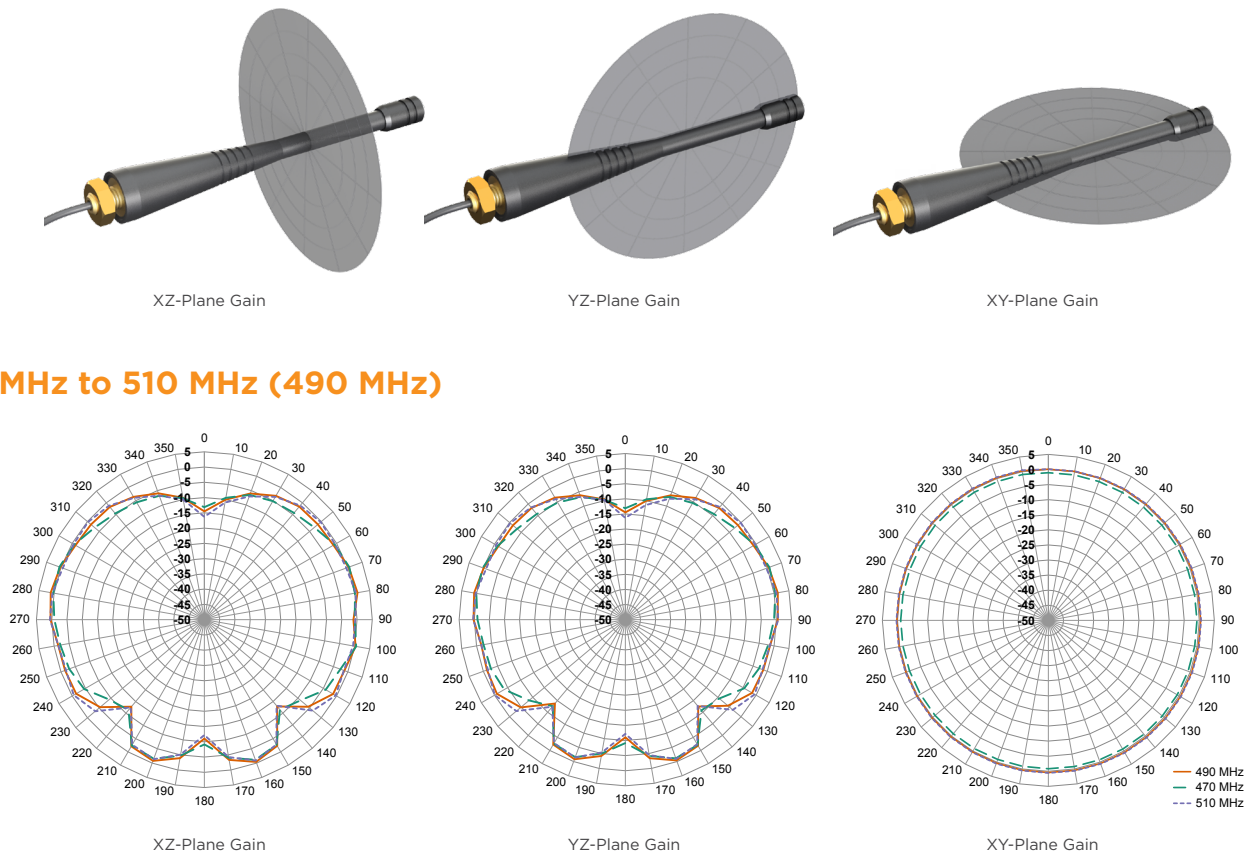
Figure 8. Radiation Patterns for PW 490 MHz Antenna
