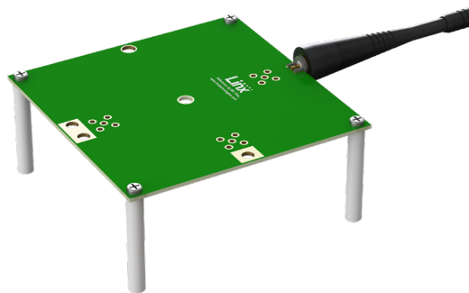
Figure 7. PW 490 MHz Antenna Shown On Edge of Ground Plane
