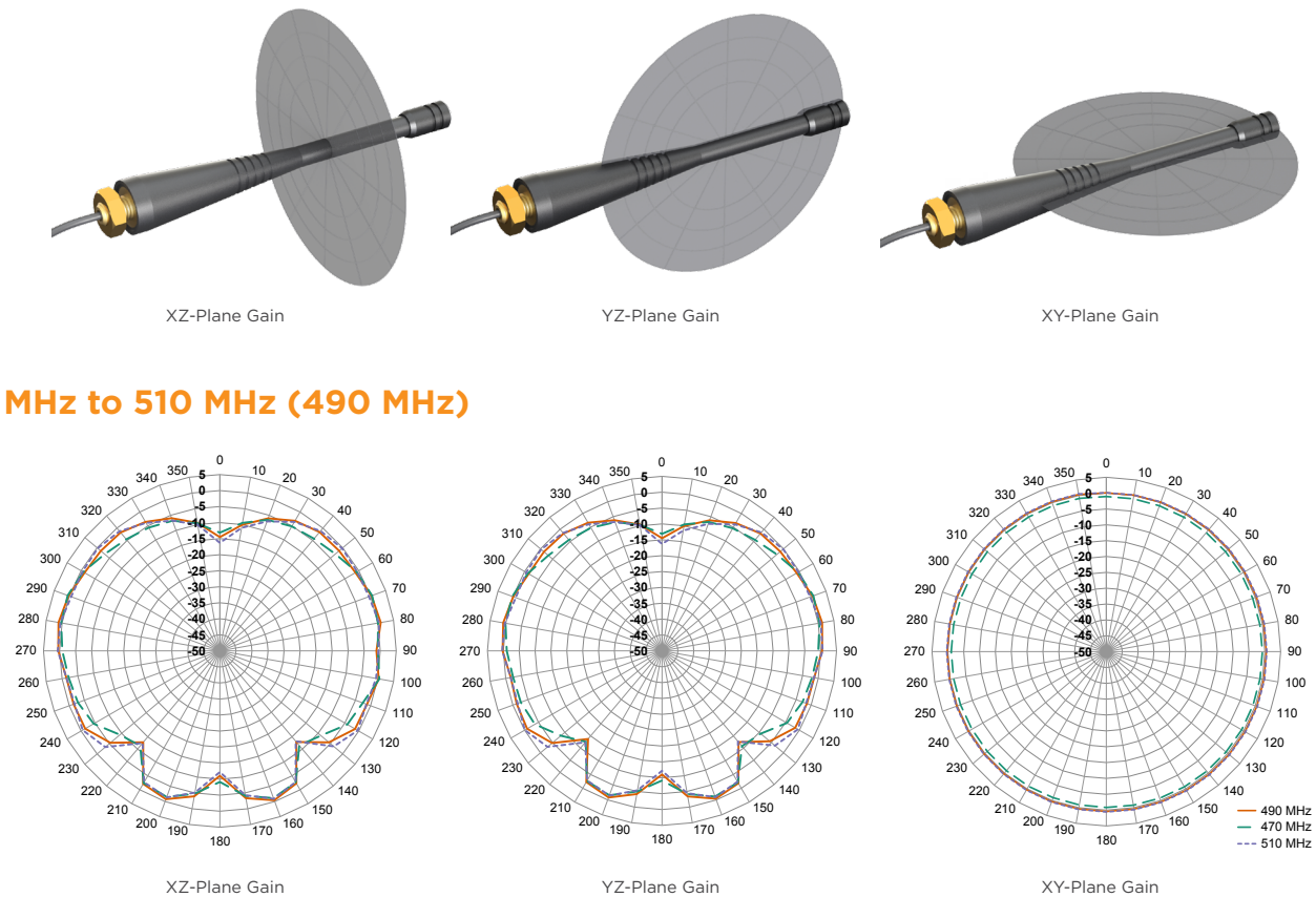
Figure 8. Radiation Patterns for PW 490 MHz Antenna
