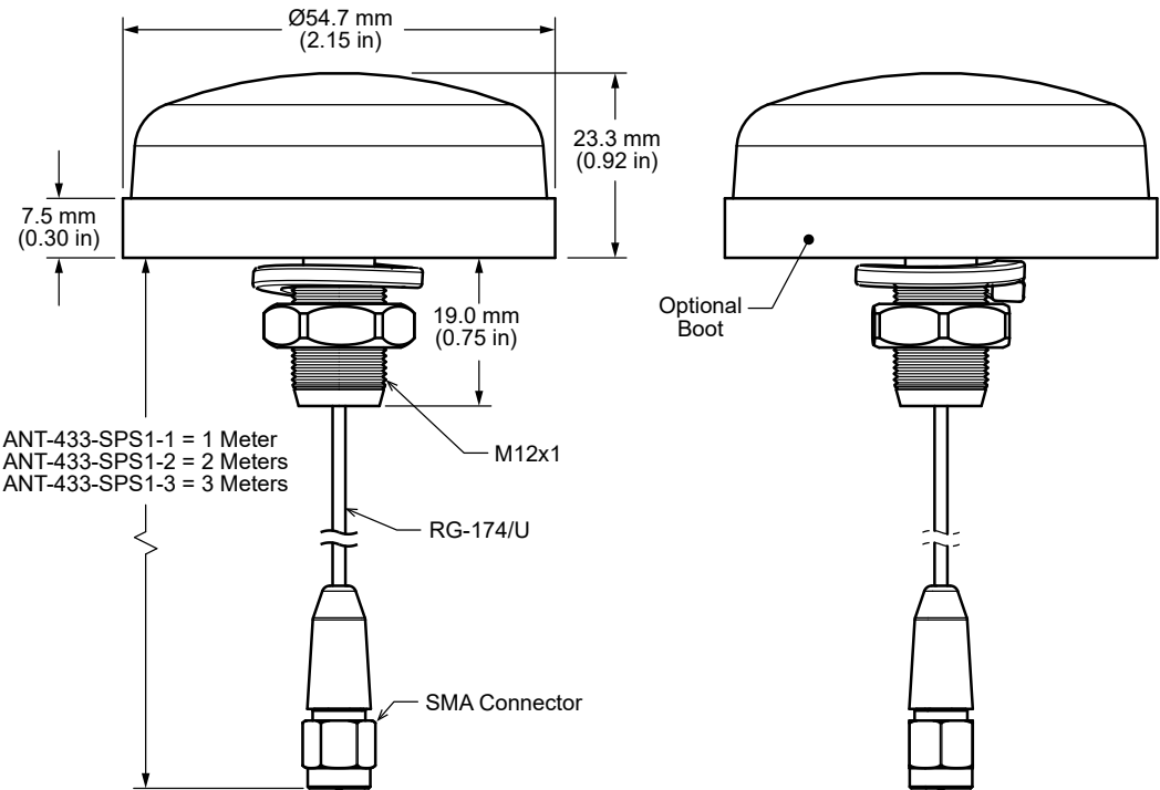
Figure 1. ANT-433-SPS1 Dimensions
