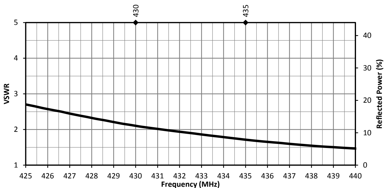
Figure 3. ANT-433-OC-LG VSWR
