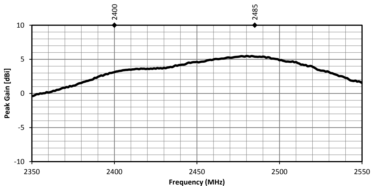
Figure 4. 2.4-CPA Peak Gain
