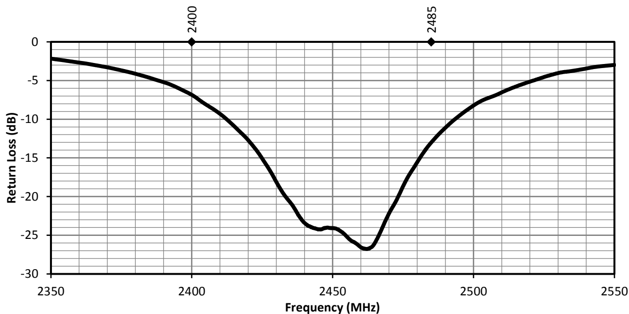
Figure 3. 2.4-CPA Return Loss
