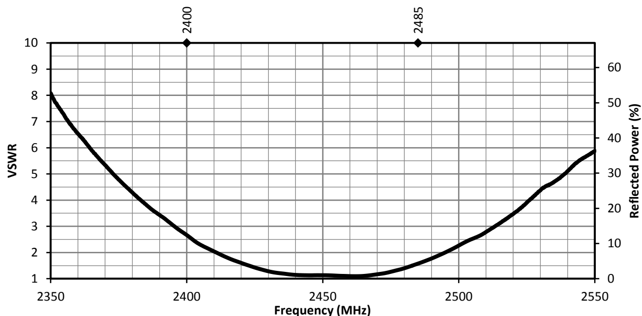
Figure 2. 2.4-CPA VSWR
