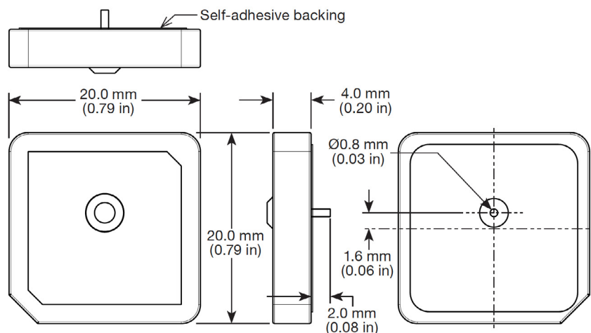
Figure 1. 2.4-CPA Antenna Dimensions
