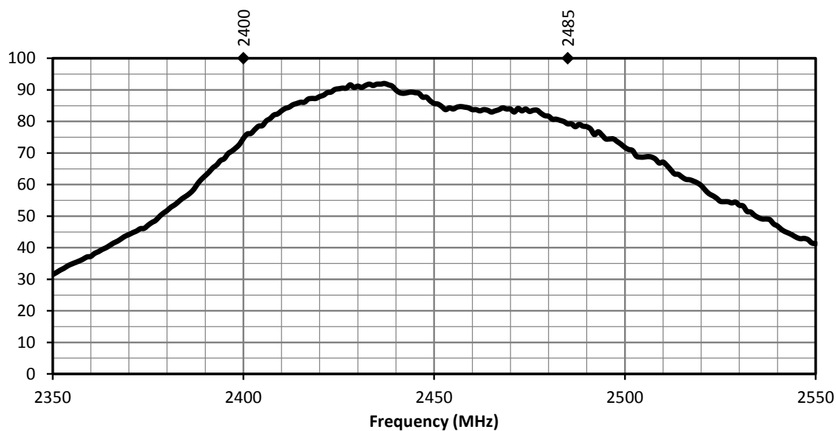
Figure 5. 2.4-CPA Antenna Radiation Efficiency
