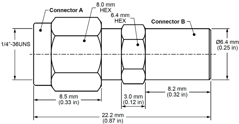
Figure 1. Product Dimensions for the ADP-SMAM-SMBM-G Adapter
