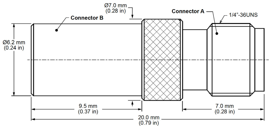
Figure 1. Product Dimensions for the ADP-SMAF-SMBM-G Adapter
