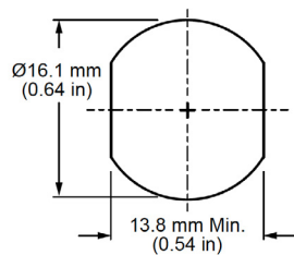
Figure 2. Recommended Enclosure Mounting Dimensions
