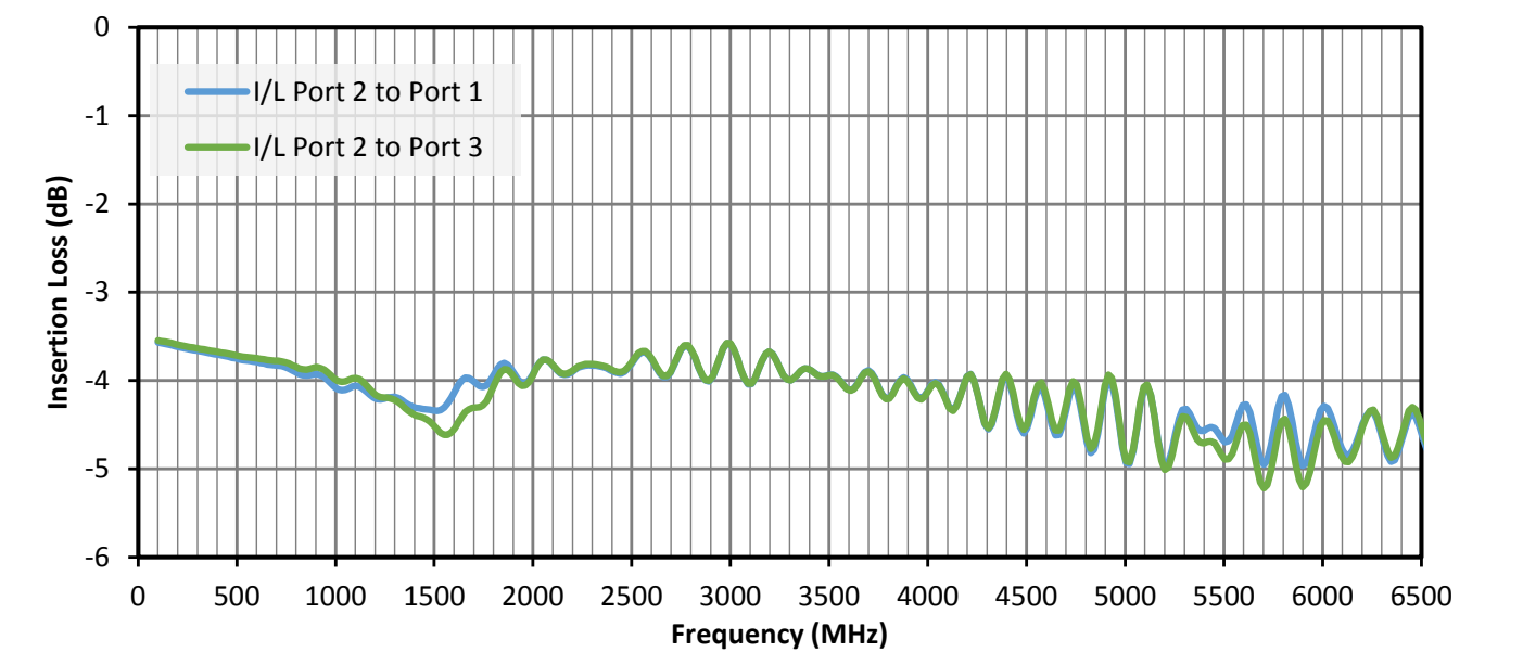
Figure 2. Insertion Loss for the ADP-BNCM-BNCF-T Adapter
