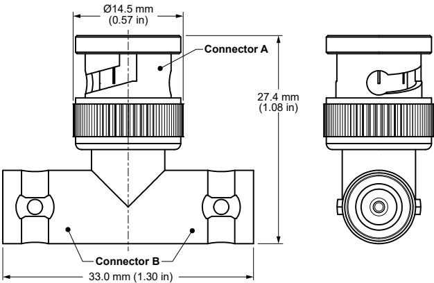
Figure 1. Product Dimensions for the ADP-BNCM-BNCF-T Adapter
