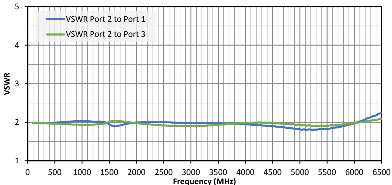
Figure 3. VSWR for the ADP-BNCM-BNCF-T Adapter
