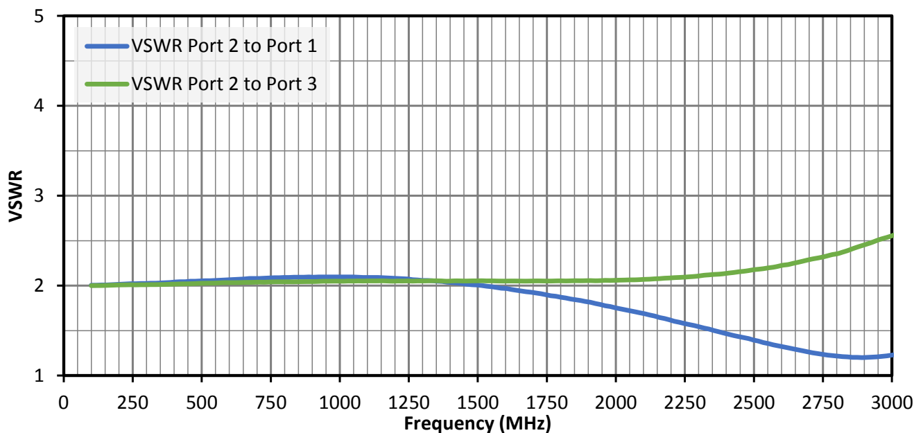
Figure 3. VSWR for the ADP-BNCF-T-2 Adapter
