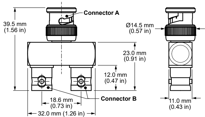
Figure 1. Product Dimensions for the ADP-BNCM-BNCF-T-2 Adapter
