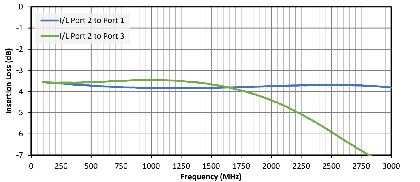
Figure 2. Insertion Loss for the ADP-BNCM-BNCF-T-2 Adapter
