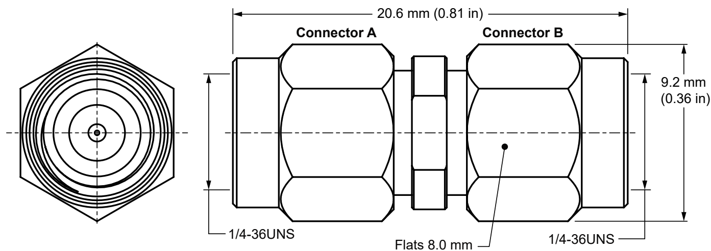
Figure 1: Product Dimensions for the ADP-2.92M-2.92M Adapter
