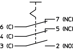
2 NC / 1 NO
