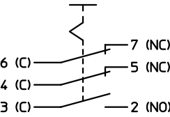
2 NC / 1 NO
