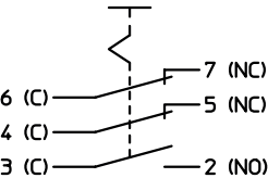
2 NC / 1 NO
