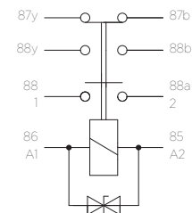
NO-Contact/Auxiliary-Contact
