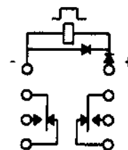
TERMINAL VIEW
